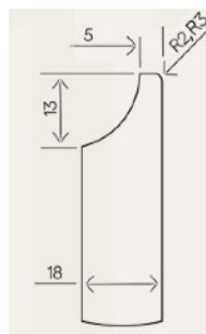
Z2 (RADIUS r2mm nebo r3mm)
